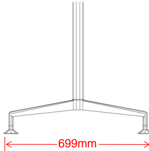
8400 small table legs
